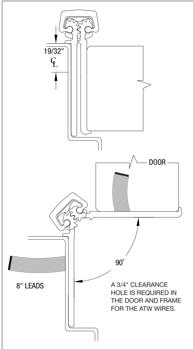
4-PIN AND 8-PIN CONNECTORS ARE SUPPLIED ON THE END OF 8" LEADS.
