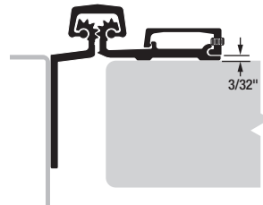
SAFETY HINGE APPLICATION
